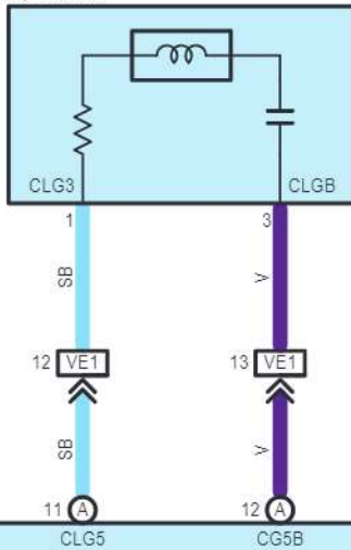
V3 Front Indoor Electrical Key Oscillator
