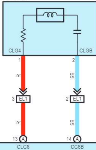
L8 Rear Indoor Electrical Key Oscillator
