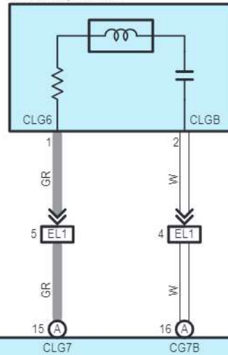
L9 Indoor Luggage Compartment Electrical Key Oscillator
