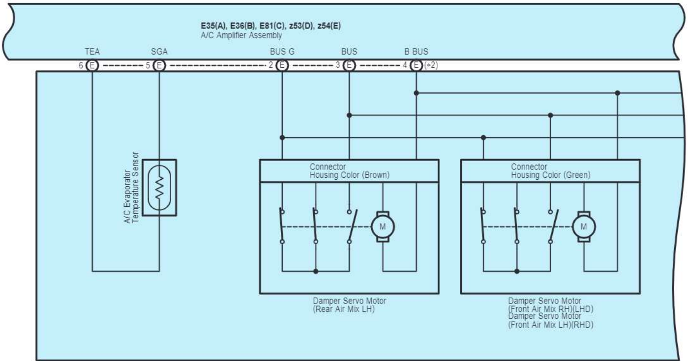
z54(E) A/C Blower Assembly
